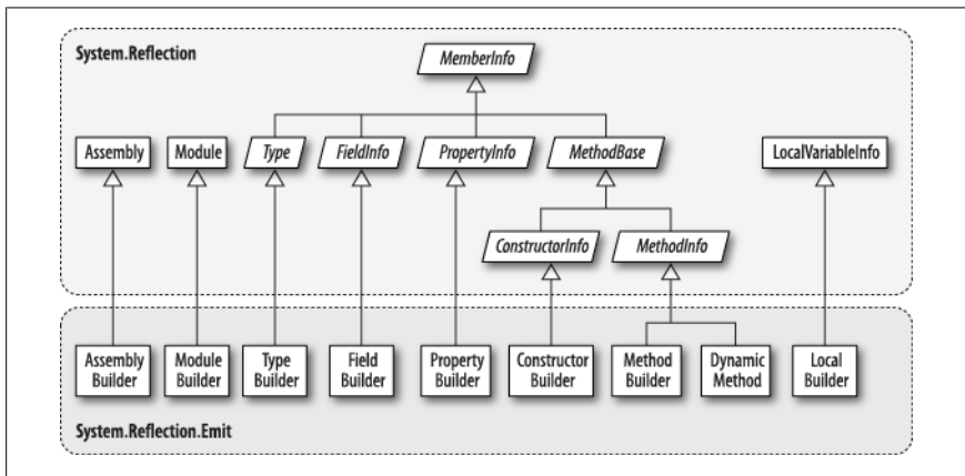
Figure 19-2. System.Reflection.Emit
