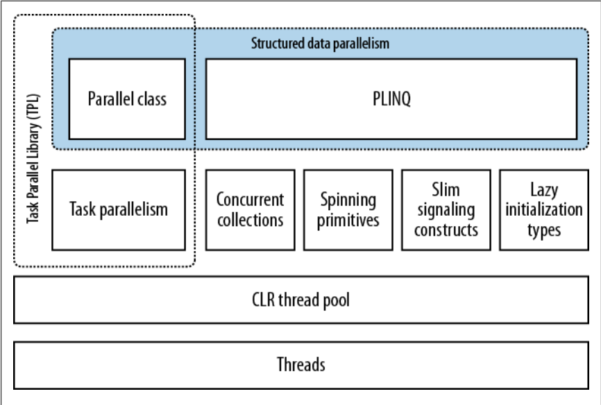
Figure 23-1. PFX components
