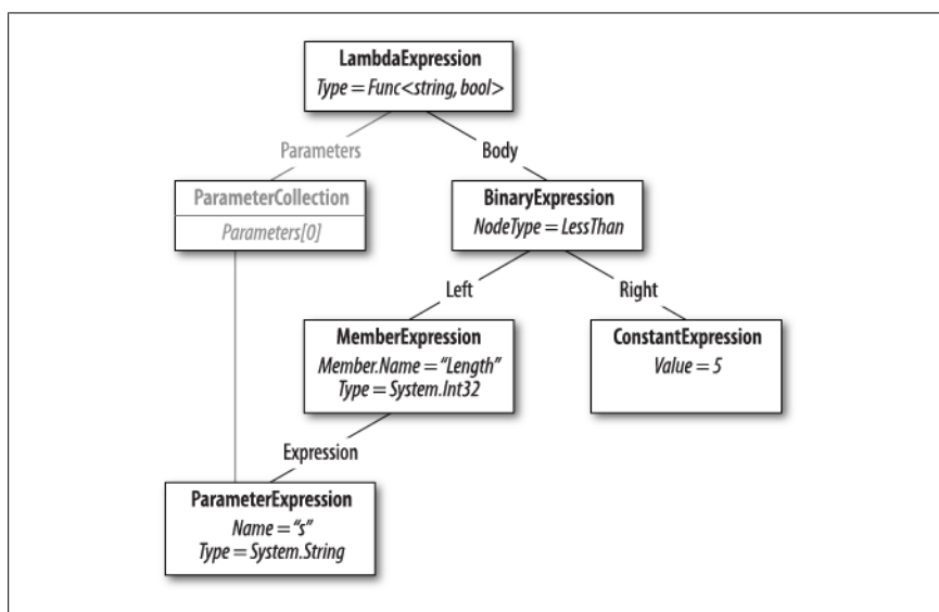
Figure 8-11. Expression tree
