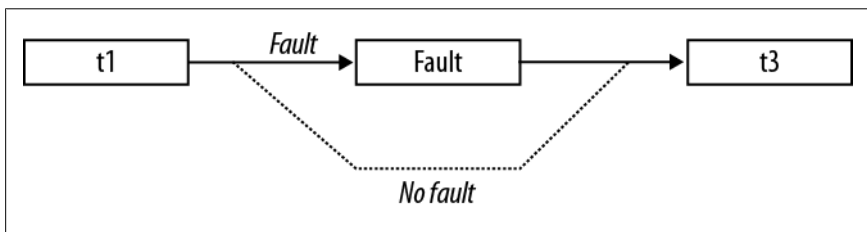
Figure 23-6. Conditional continuations
