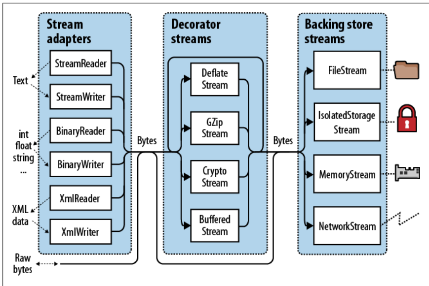
Figure 15-1. Stream architecture
