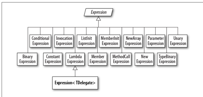
Figure 8-10. Expression types
