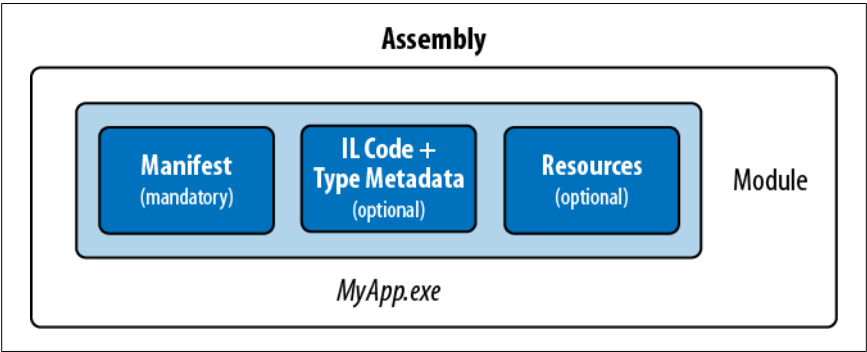
Figure 18-1. Single-file assembly
