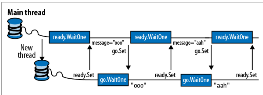
Figure 22-2. Two-way signaling
