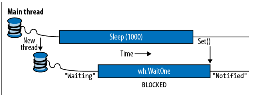
Figure 22-1. Signaling with an EventWaitHandle
