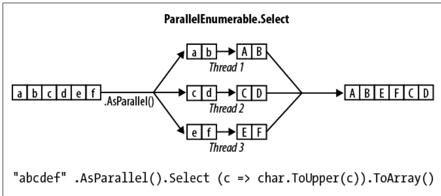
Figure 23-2. PLINQ execution model
