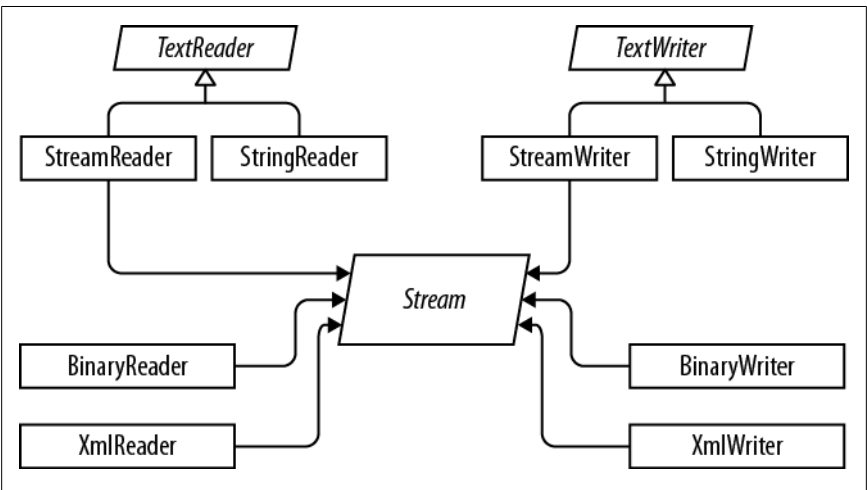
Figure 15-5. Readers and writers
