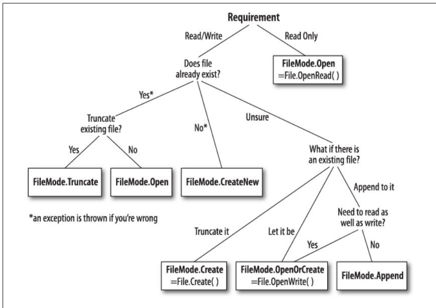
Figure 15-3. Choosing a FileMode
