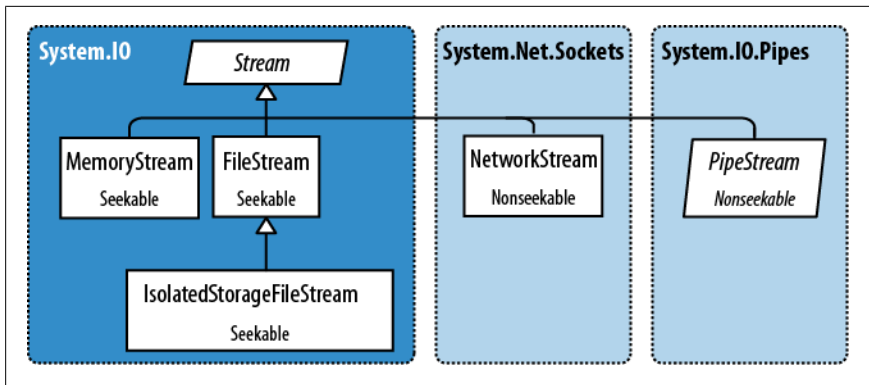
Figure 15-2. Backing store streams
