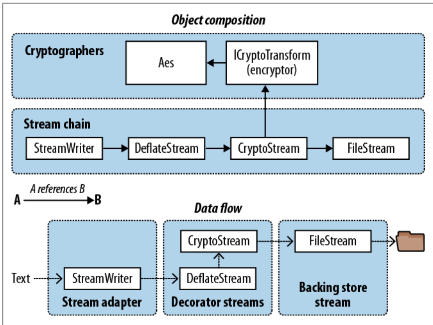
Figure 21-2. Chaining encryption and compression streams
