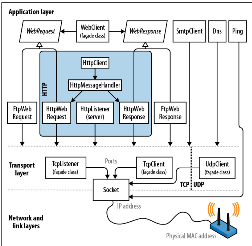
Figure 16-1. Network architecture
