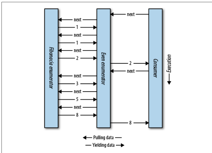
Figure 4-1. Composing sequences
