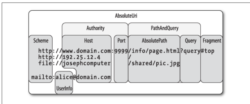
Figure 16-2. URI properties
