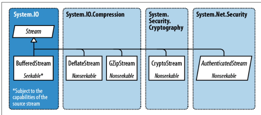
Figure 15-4. Decorator streams
