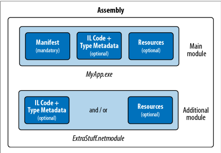
Figure 18-2. Multifile assembly
