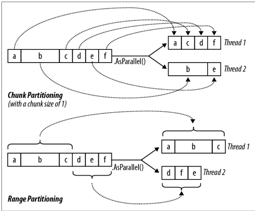
Figure 23-4. Chunk versus range partitioning
