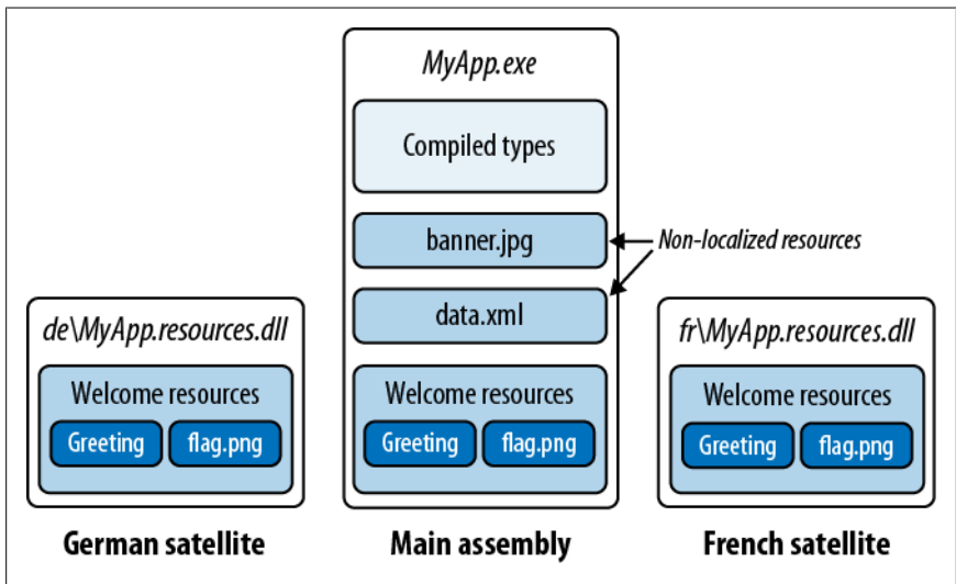
Figure 18-4. Resources
