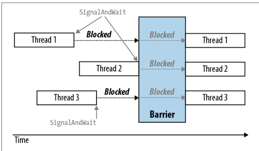
Figure 22-3. Barrier
