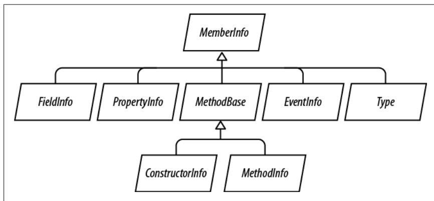
Figure 19-1. Member types
