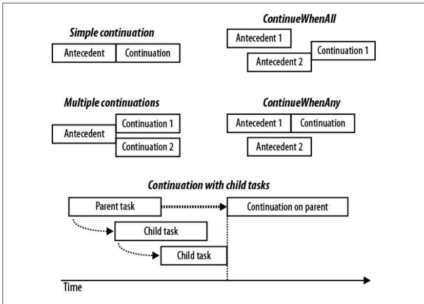
Figure 23-5. Continuations
